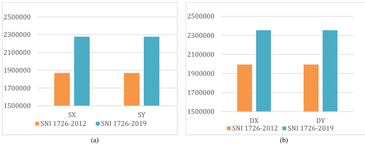
Figure 5. Basic Shear Force
