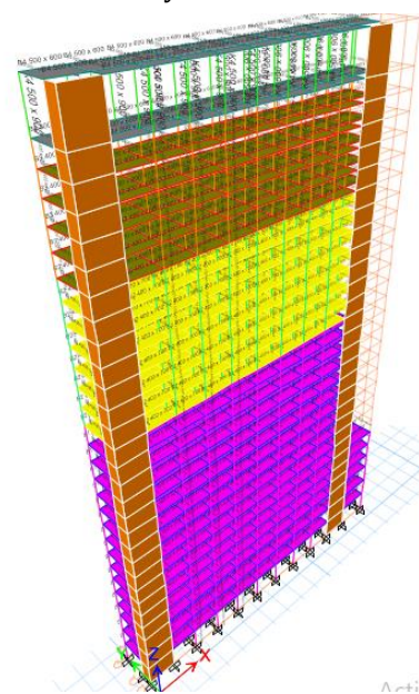
Figure 1. Modeling Structure 3-D
