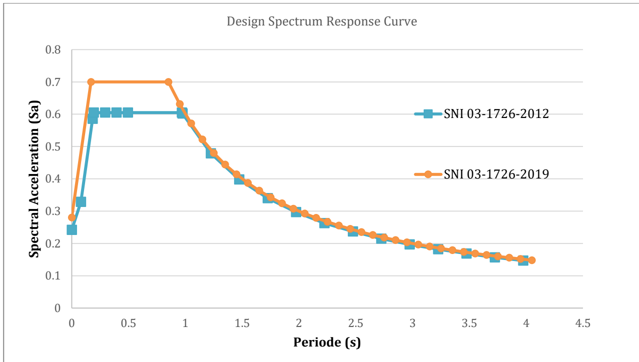
Figure 3. Design Spectrum Response Curve
