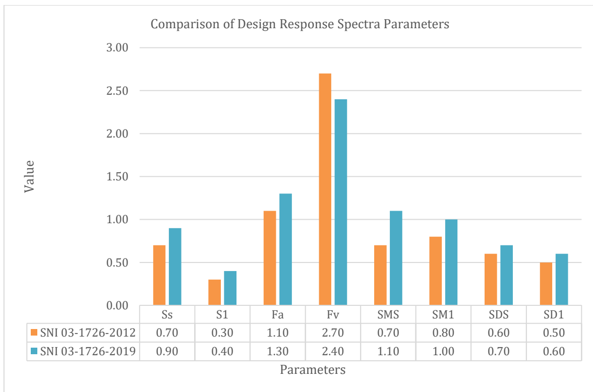
Figure 2. Comparison of Design Response Spectra Parameters
